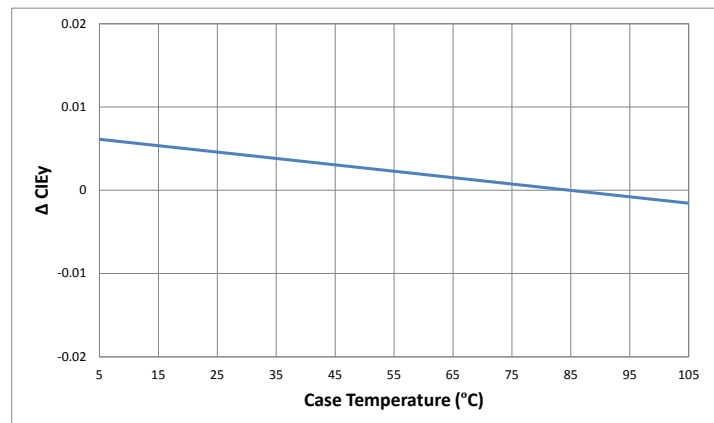
Change in CIE y vs. Case Temperature (3000K, 80CRI)
