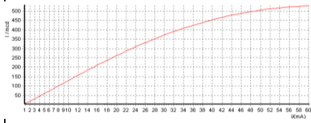
Current-Luminous intensity Curve
