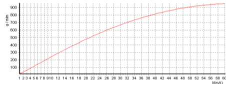
Current-Luminous flux Curve
